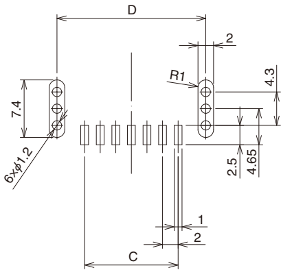
◆Recommended PCB pattern
