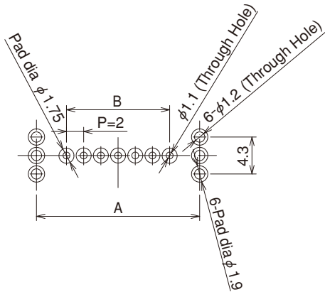
Recommended PCB pattern and Pin No.
