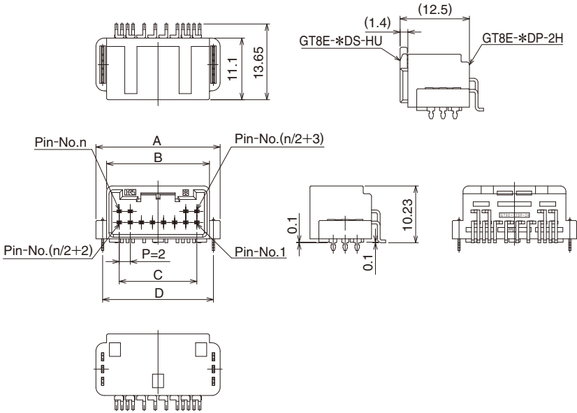
Fitting diagram
