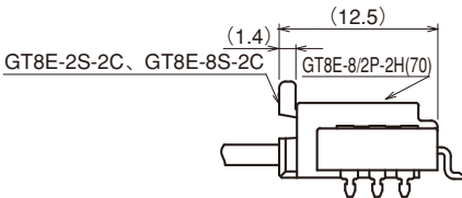
Fitting diagram
