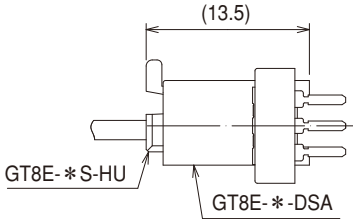
Fitting diagram
