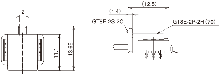
Fitting diagram
