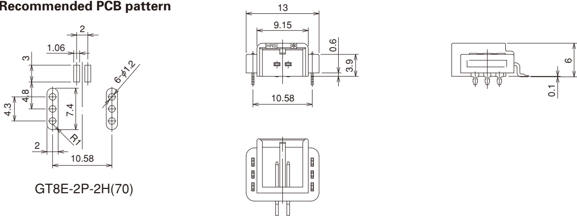
Recommended PCB pattern
