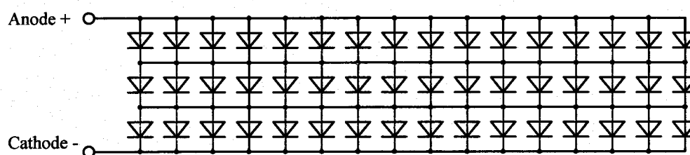
Equivalent circuit
