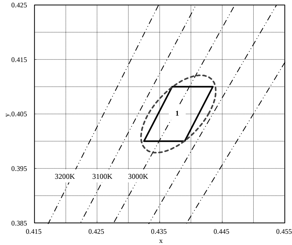
Chromaticity Diagram
