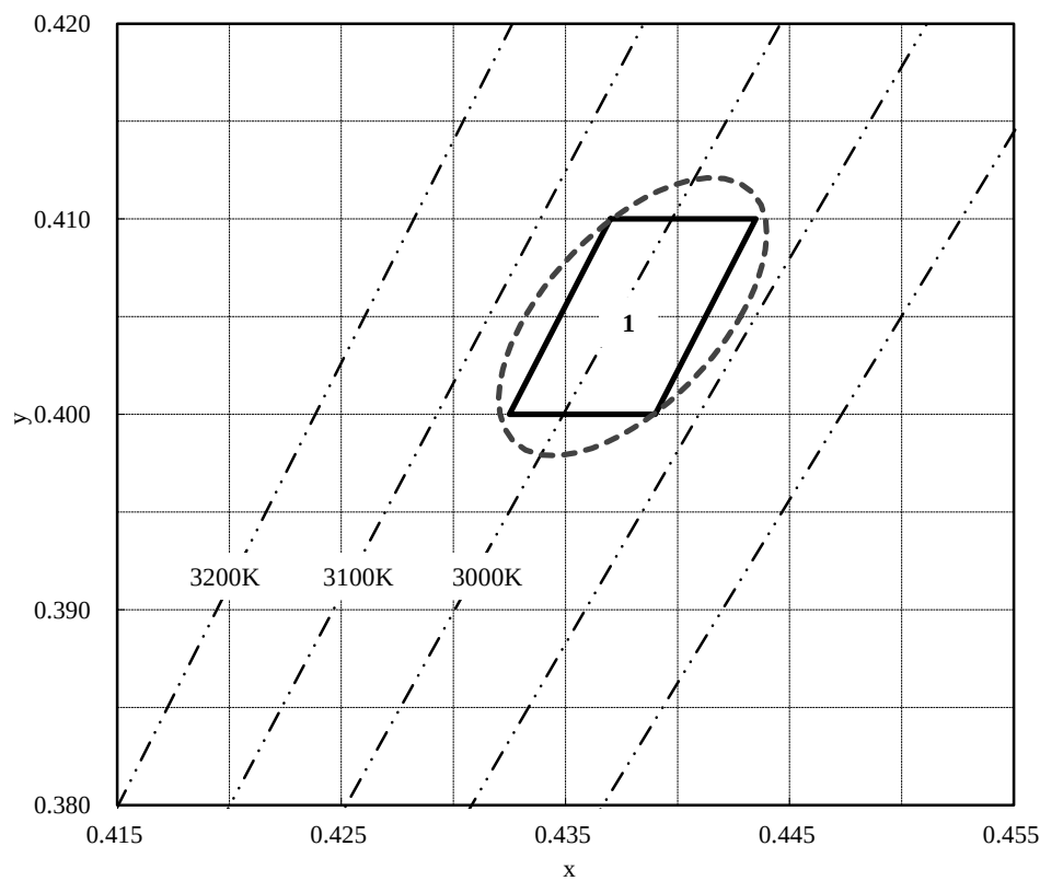
Chromaticity Diagram
