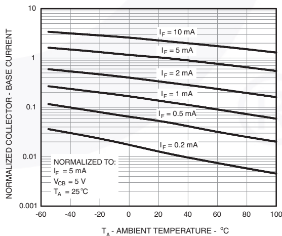
Figure 8. Normalized Collector-Base Current vs. Temperature
