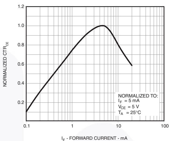
Figure 4. Normalized Current Transfer Ratio vs. Forward Current
