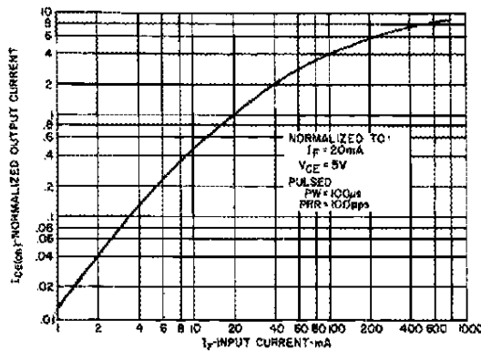
Fig. 1. Output Current vs. Input Current ST1129-11
