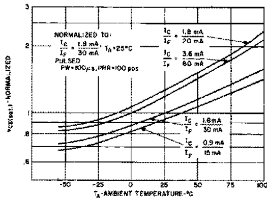
Fig. 3. V_{CE(sat)} vs. Temperature ST1130-11
