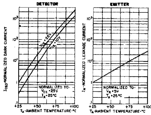
Fig. 4. Leakage Currents vs. Temperature ST1133-11
