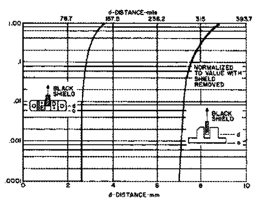
Fig. 6. Output Current vs. Distance ST1132-11
