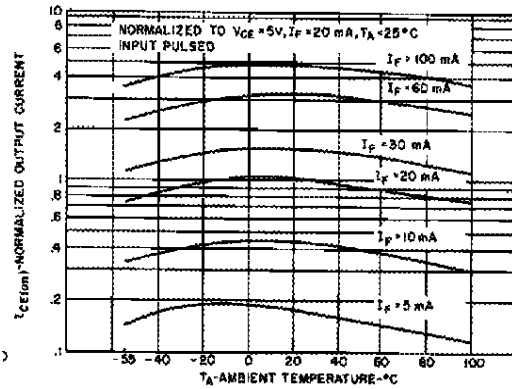
Fig. 2. Output Current vs. Temperature ST1134-11
