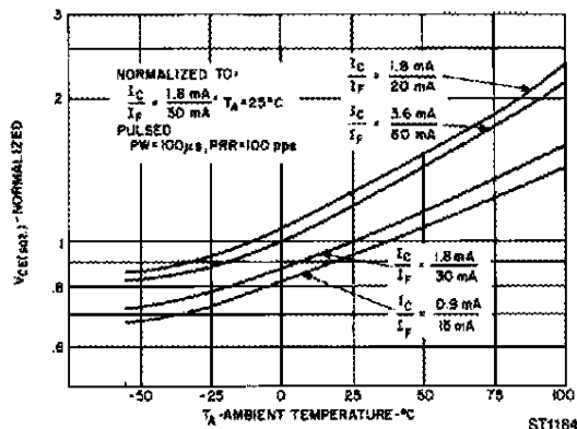
Fig. 3. V_{CE(ON)} vs. Temperature
