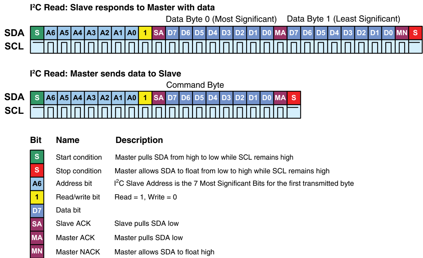
Figure 9. Sensor I 2 C Read and Write Sequences
