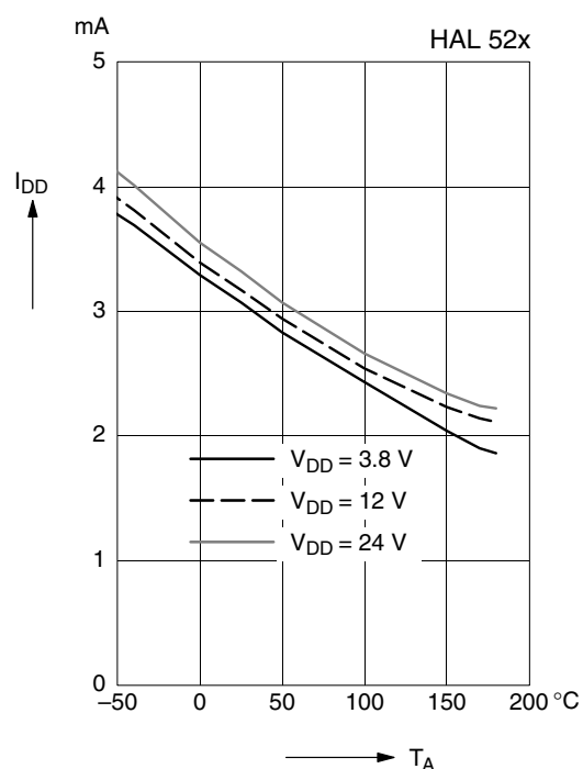
Fig. 3-9: Typical supply current versus ambient temperature
