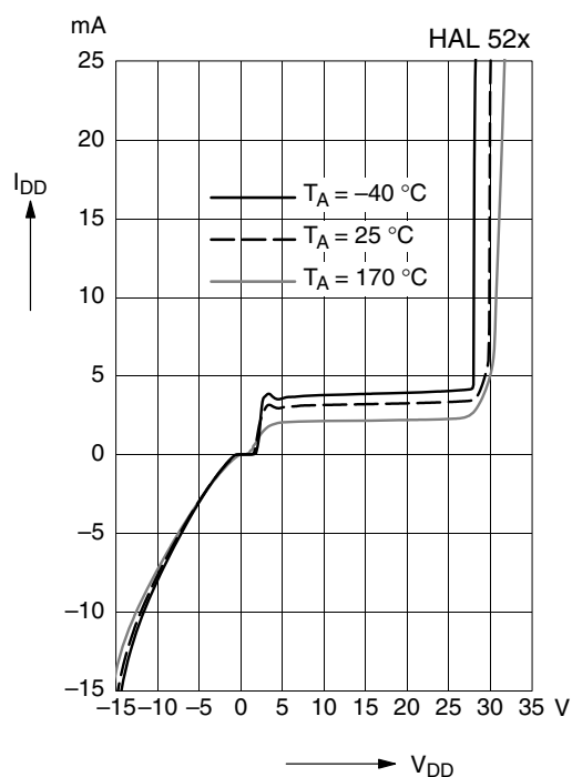
Fig. 3-7: Typical supply current versus supply voltage
