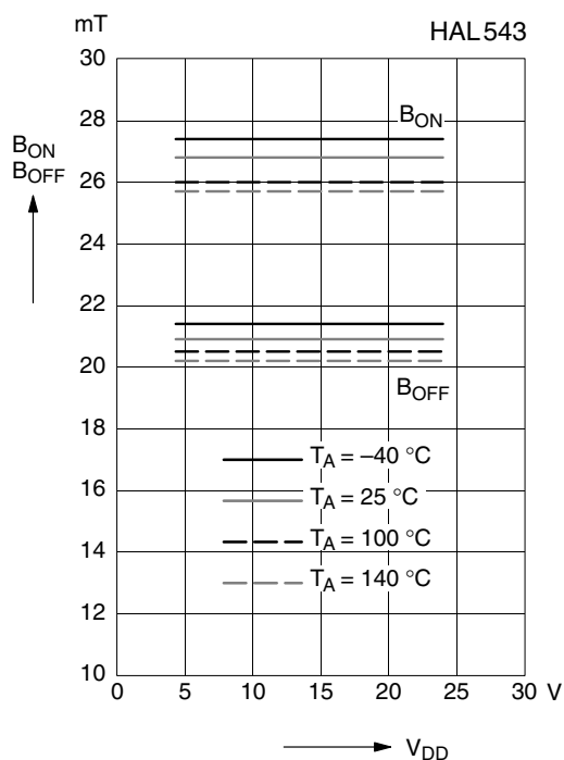
Fig. 4-5: Typ. magnetic switching points versus supply voltage
