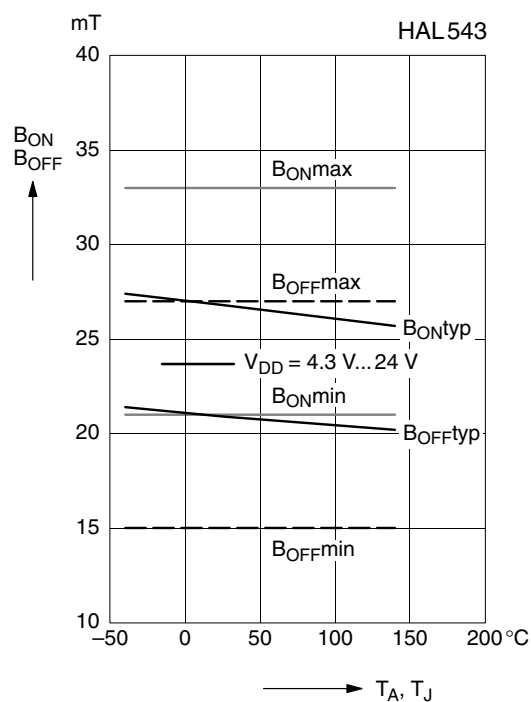
Fig. 4-6: Magnetic switching points versus temperature
