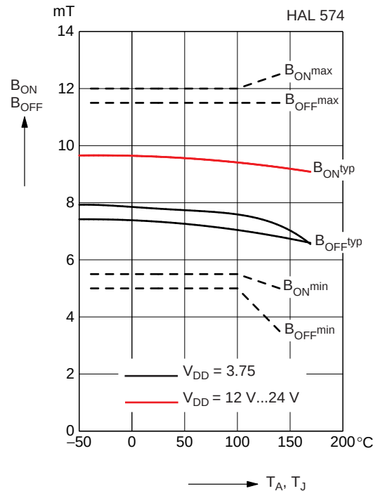
Fig. 4-8: Magnetic switching points versus temperature
