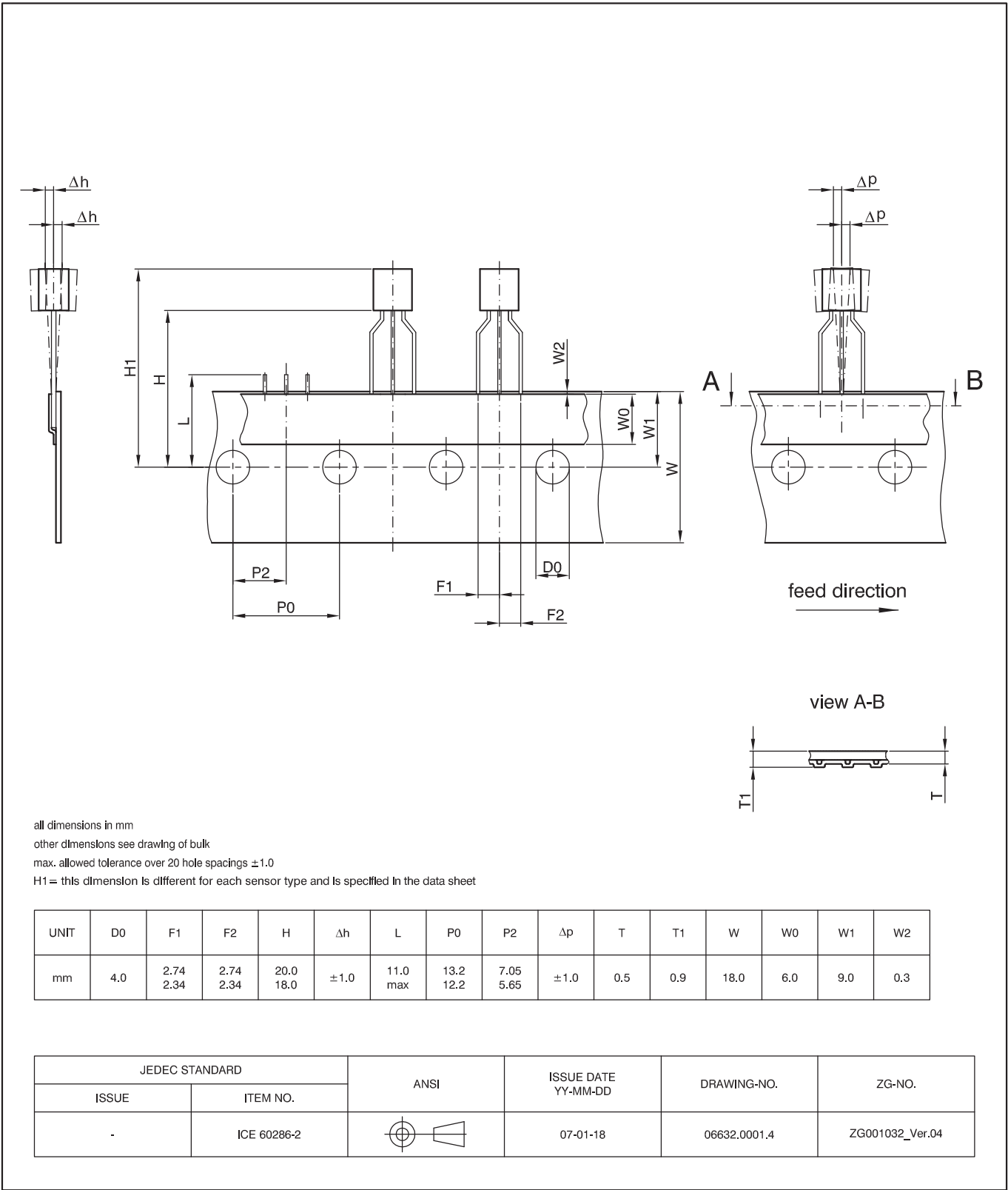
Fig. 3-5: TO92UA-1: Dimensions ammopack inline, spread
