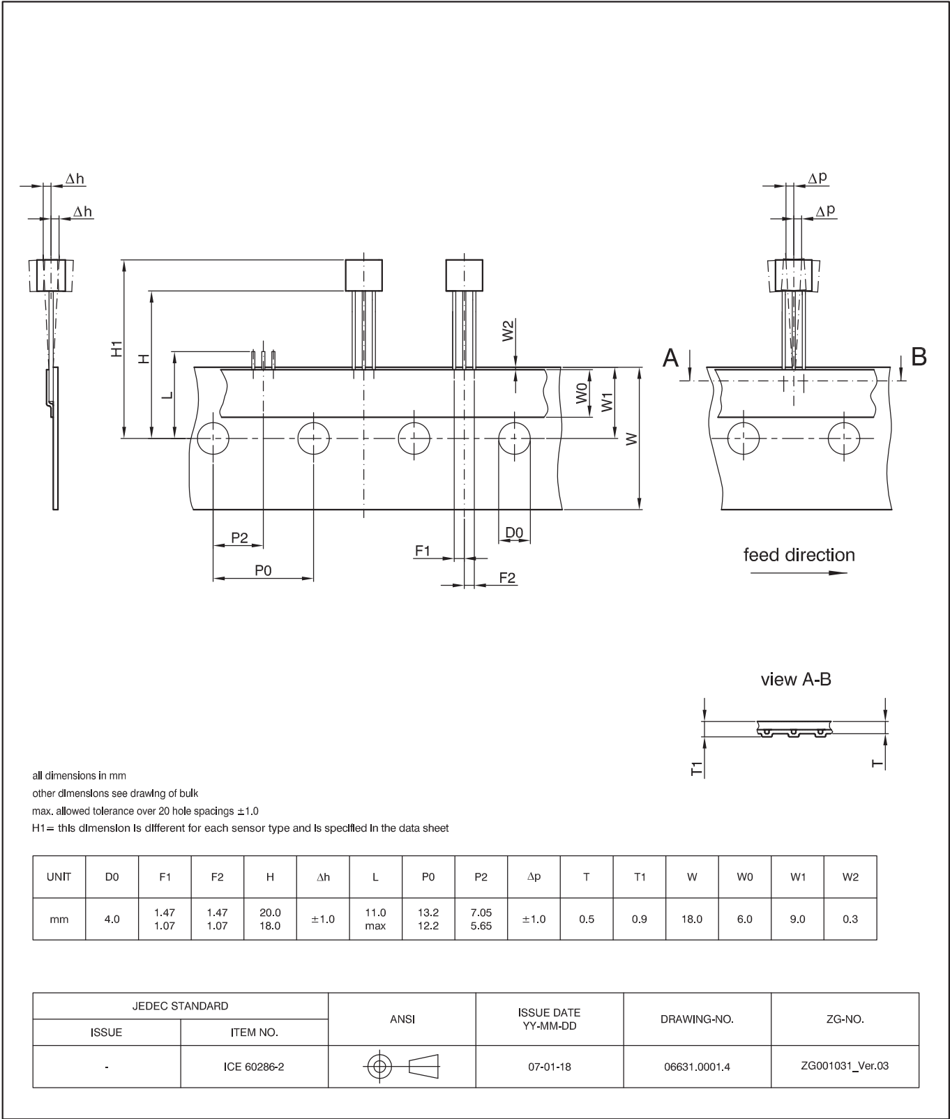
Fig. 3-4: TO92UA-2: Dimensions ammopack inline, not spread
