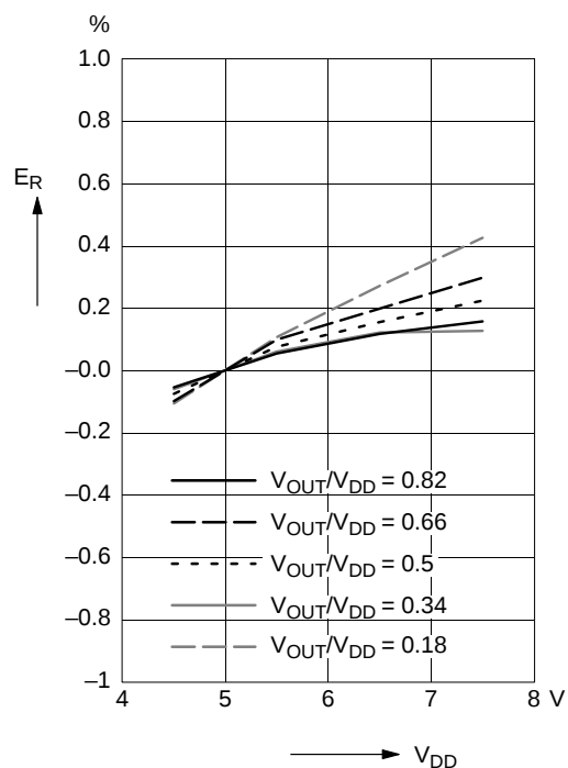
Fig. 3-6: Typical ratiometric error versus supply voltage
