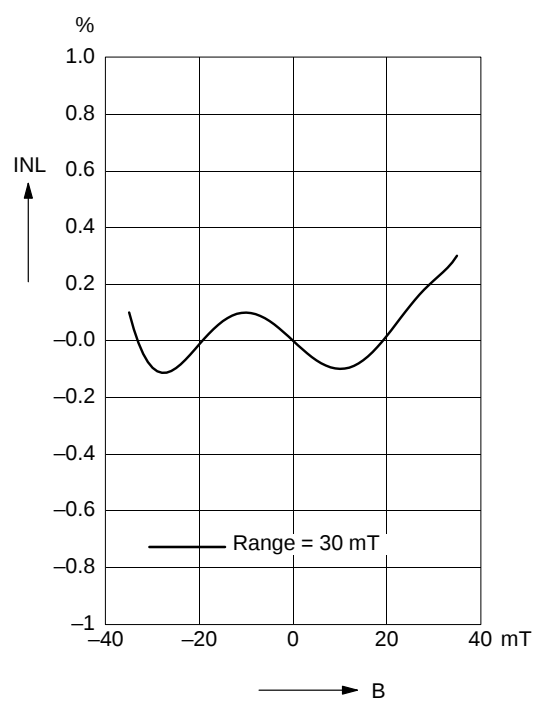
Fig. 3-9: Typical nonlinearity versus magnetic field
