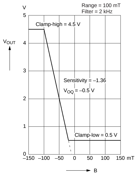
Fig. 2-5: Example for output characteristics
