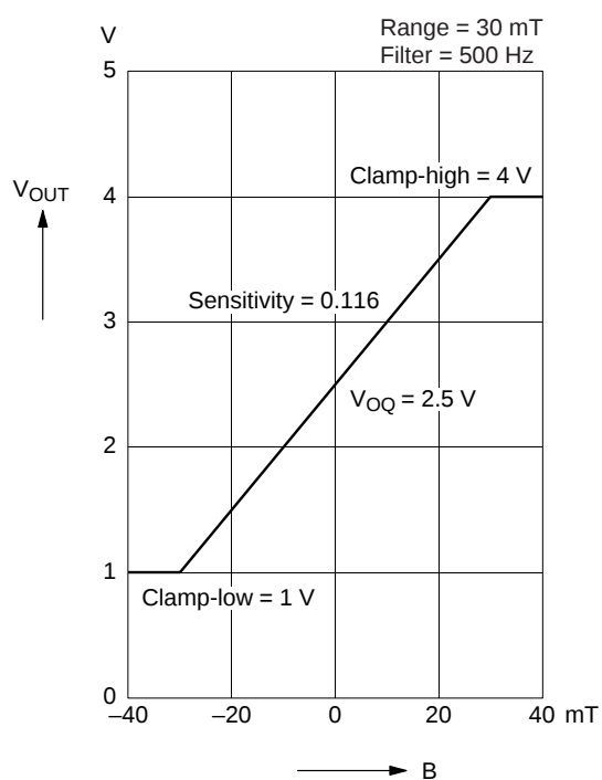
Fig. 2-4: Example for output characteristics
