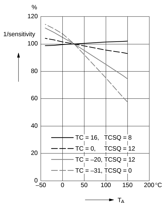
Fig. 3-7: Typical 1/sensitivity versus ambient temperature
