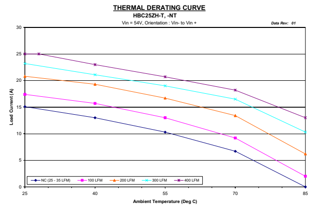
Figure 4. HBC25ZH-T, NT Derating Curves
