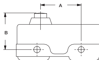
FIG. 3 Stub Plunger
