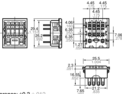
External dimensions
