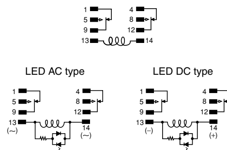
Schematic (Bottom view) Standard type
