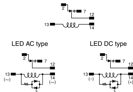
Schematic (Bottom view) Standard type
