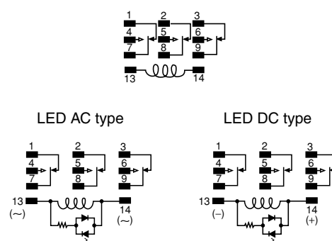
Schematic (Bottom view) Standard type
