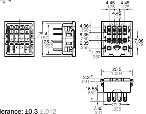
External dimensions
