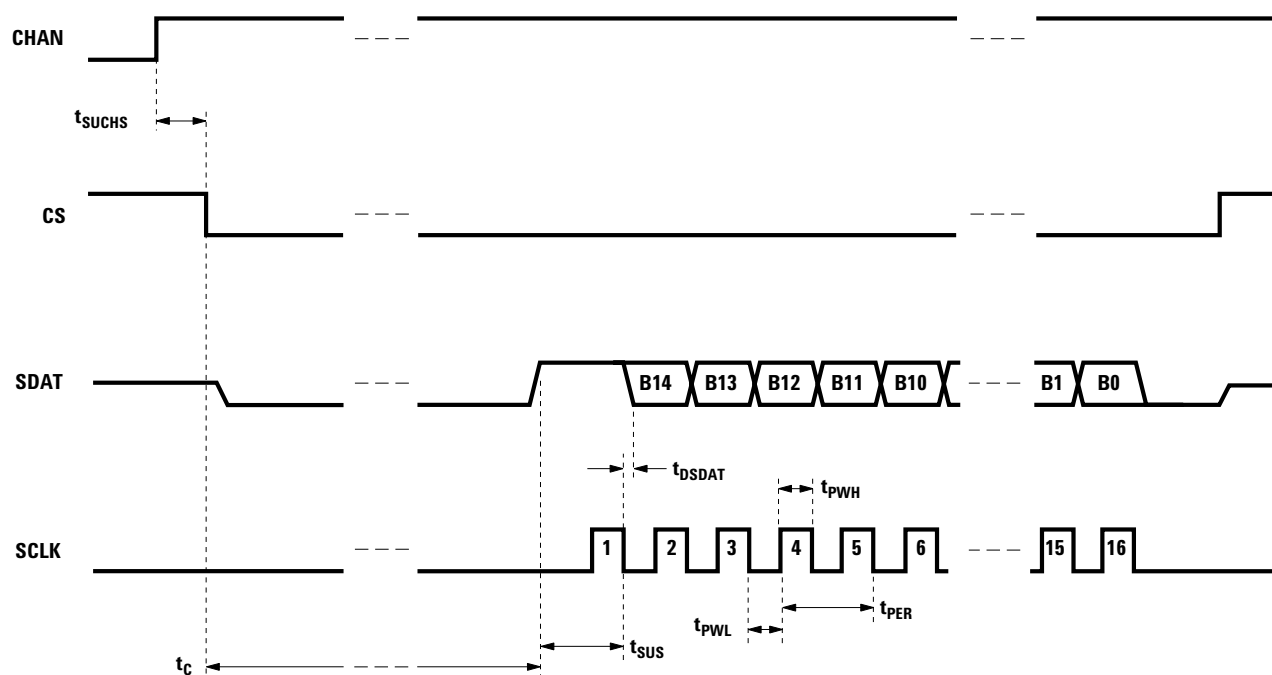
Figure 2. Conversion Timing.
