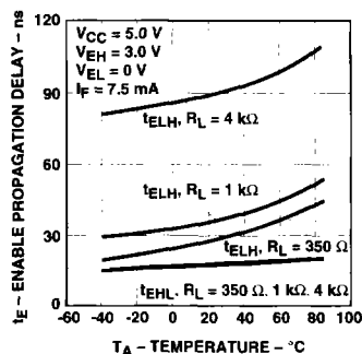
Figure 14. Typical Enable Propagation Delay vs. Temperature.
