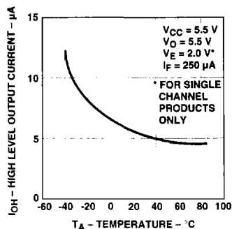
Figure 1. Typical High Level Output Current vs. Temperature.
