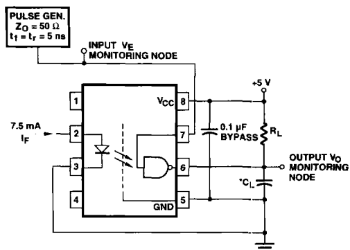
Figure 13. Test Circuit for t_{EBL} and t_{ELH} .
