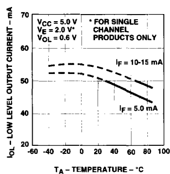
Figure 5. Typical Low Level Output Current vs. Temperature.
