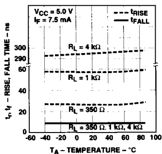
Figure 12. Typical Rise and Fall Time vs. Temperature.
