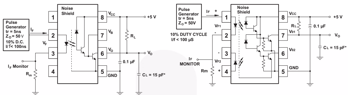
Test Circuit for 6N138, 6N139
