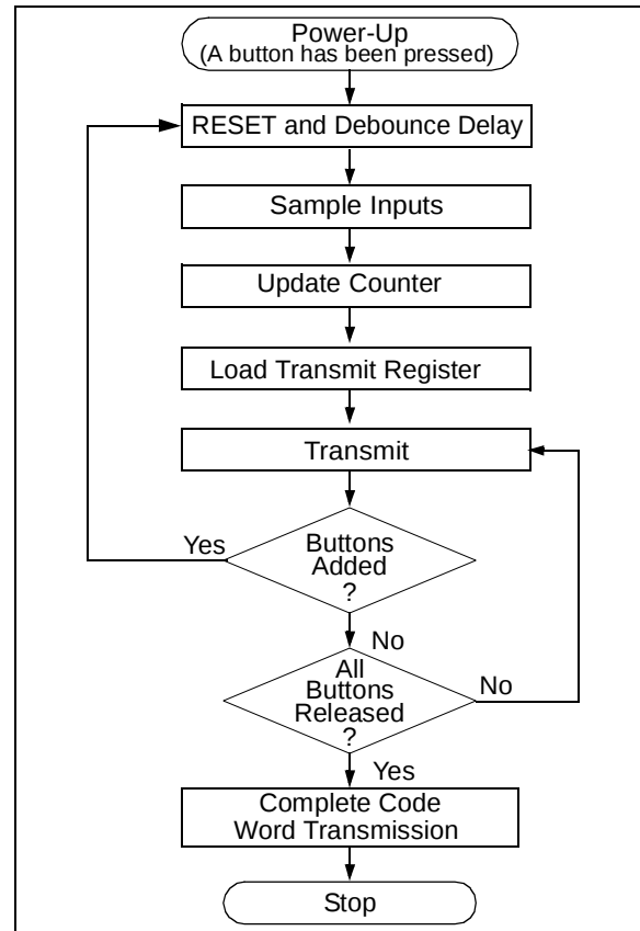
FIGURE 2-2: ENCODER OPERATION
