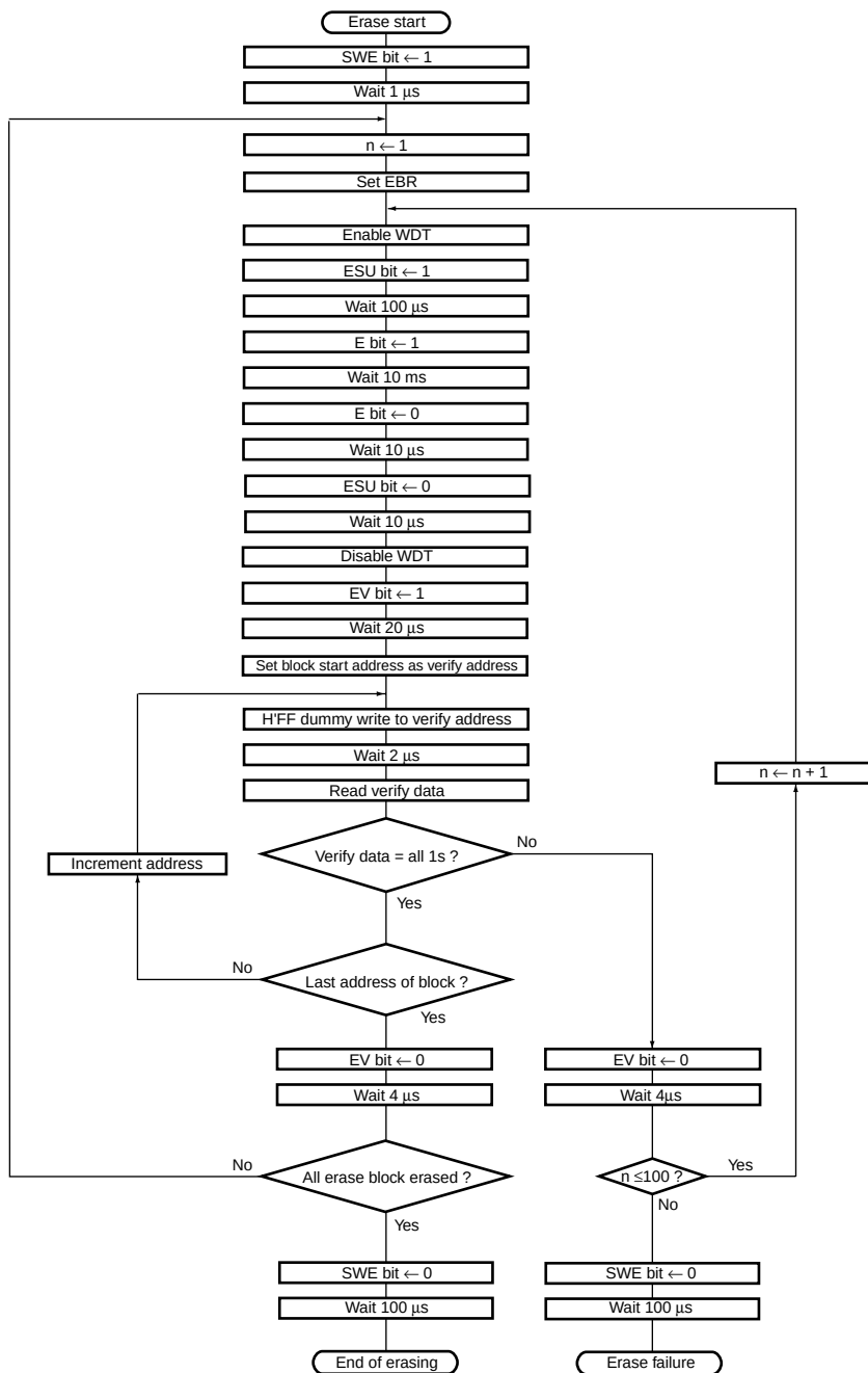
Figure 6.11 Erase/Erase-Verify Flowchart
