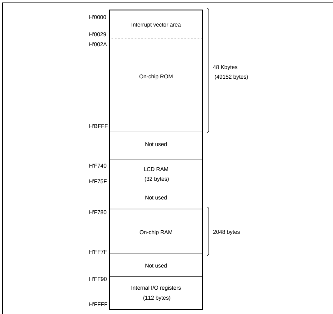
Figure 2.16 (5) H8/3826R, H8/3826S, H8/38326, and H8/38426 Memory Map
