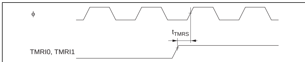
Figure 20.18 8-Bit Timer Reset Input Timing
