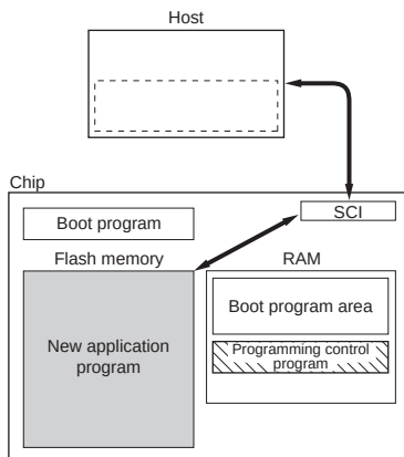
Figure 17.35 Boot Mode
