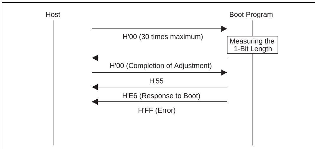
Figure 17.83 Bit-Rate-Adjustment Sequence
