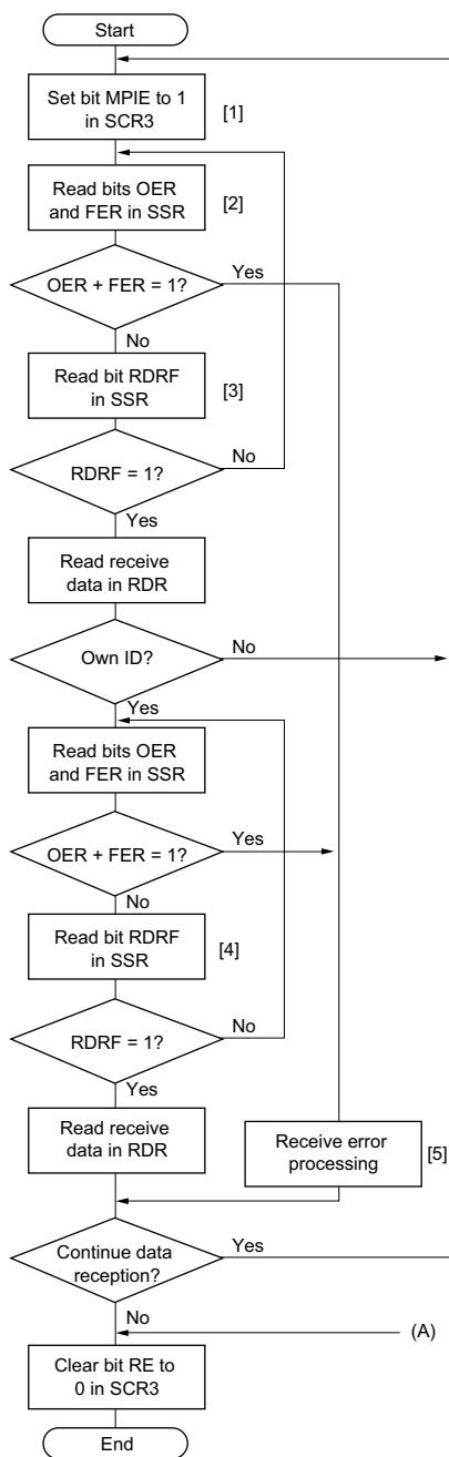
Figure 10.19 Example of Multiprocessor Data Reception Flowchart
