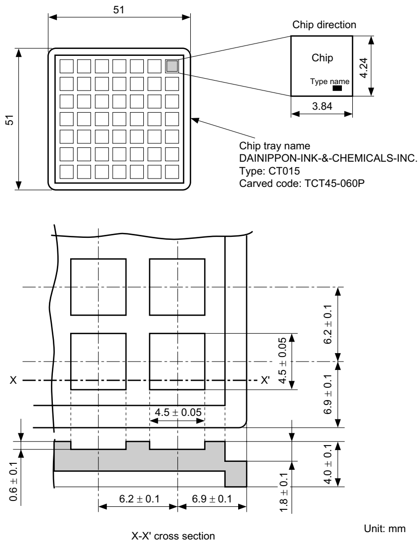
Figure I.2 Specifications of Chip Tray for the HCD64F38024 and HCD64F38024R
