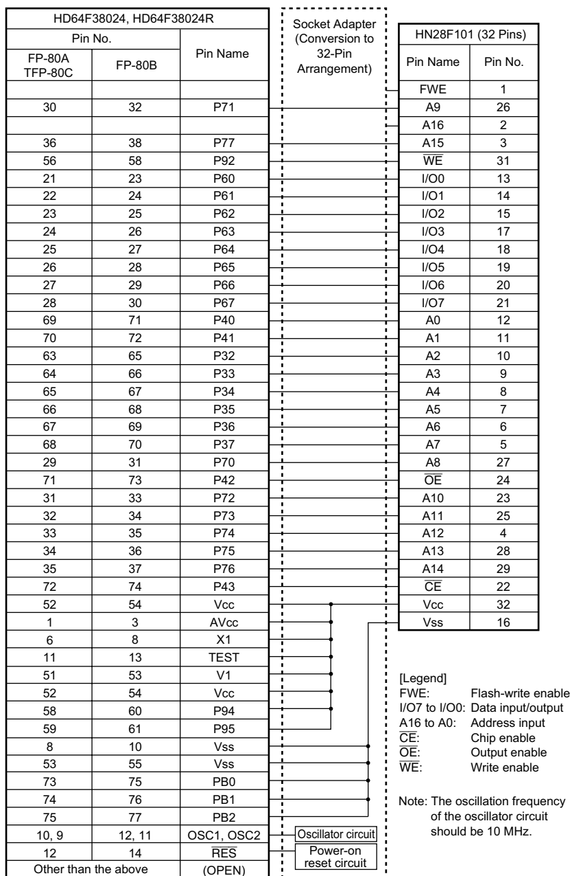
Figure 6.12(1) Socket Adapter Pin Correspondence Diagram (HD64F38024, HD64F38024R)
