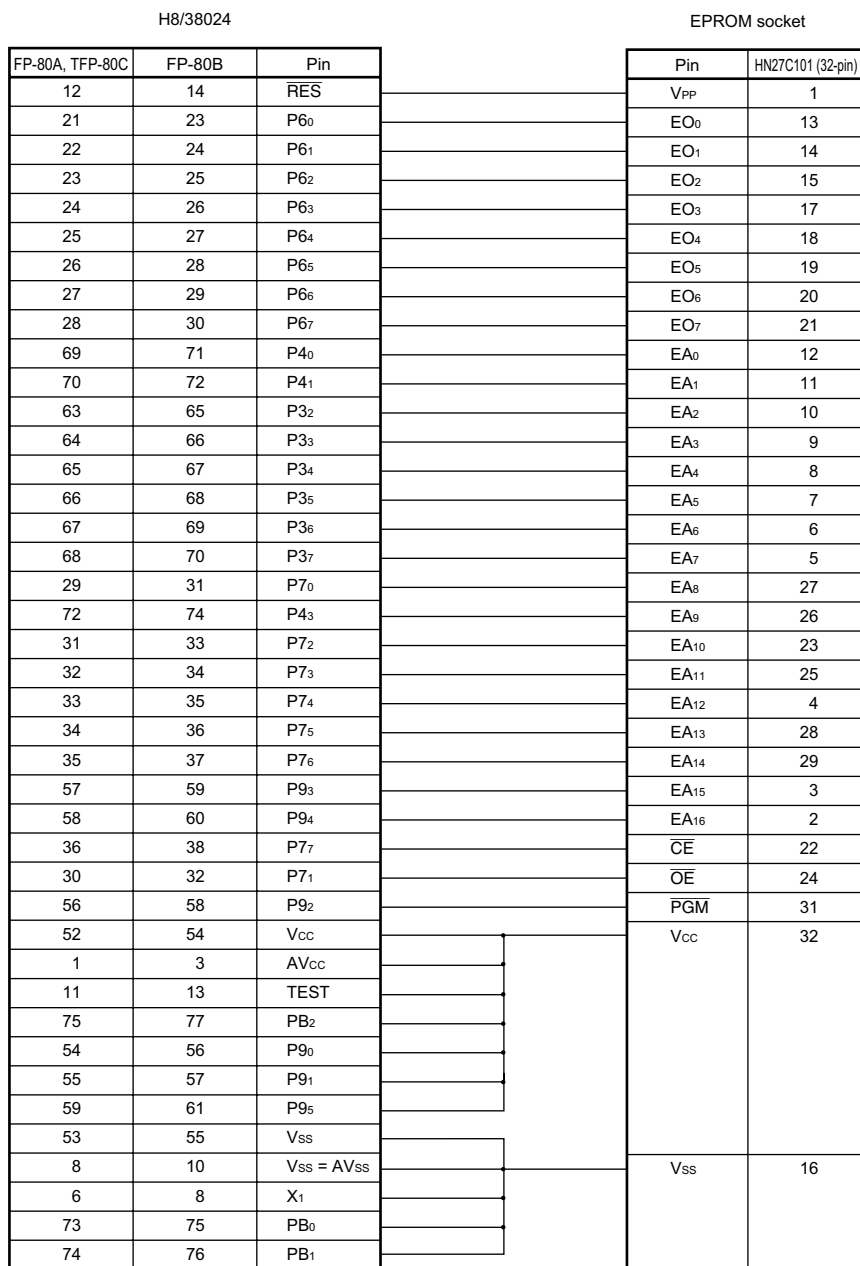
Figure 6.2 Socket Adapter Pin Correspondence (with HN27C101)
