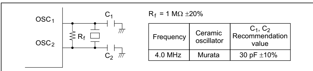
Figure 4.5(1) Typical Connection to Ceramic Oscillator (H8/38024, H8/38024R Group)
