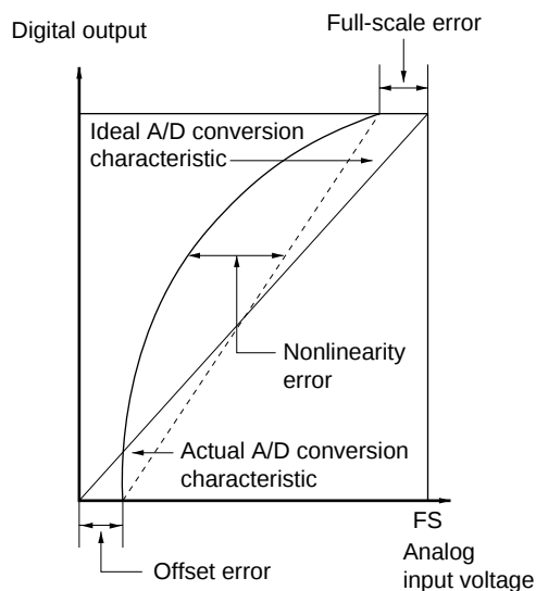
Figure 12.7 A/D Conversion Accuracy Definitions (2)
