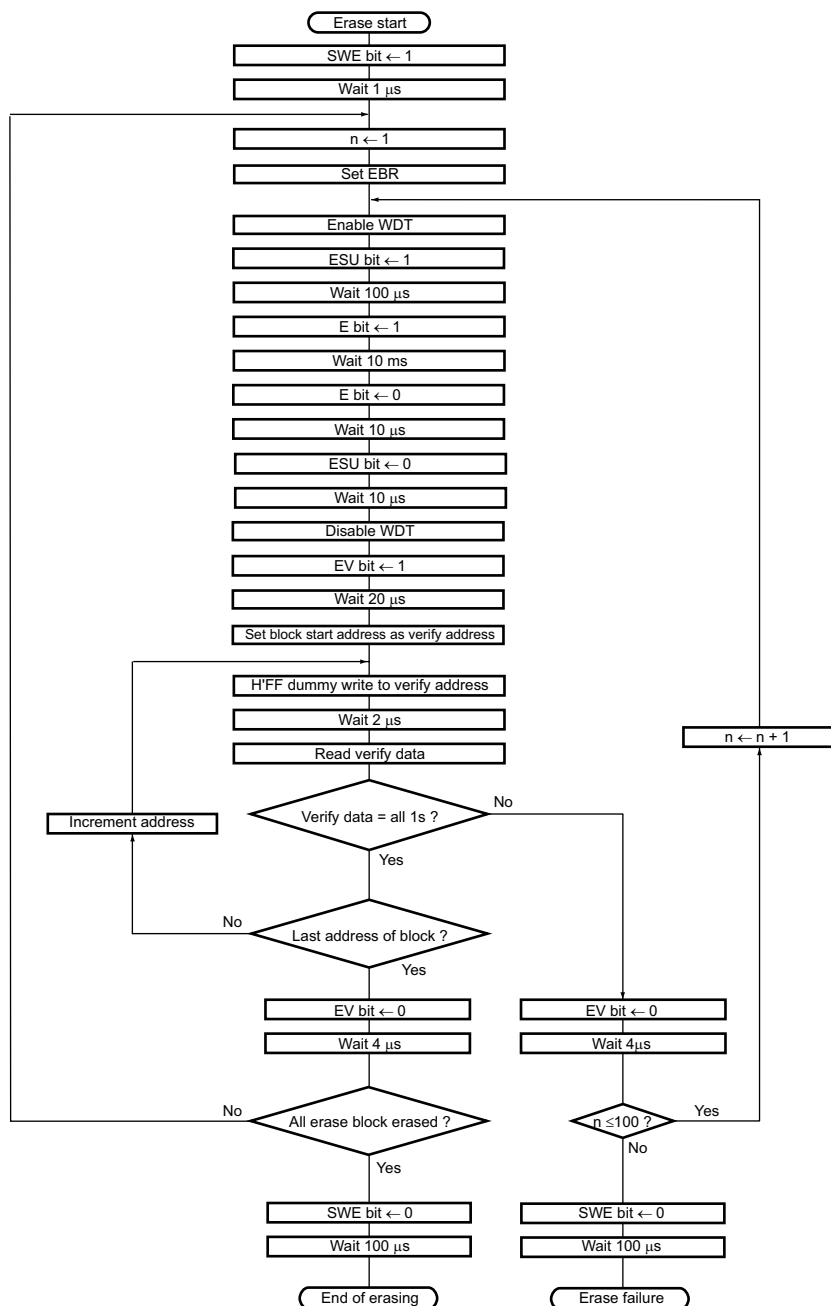
Figure 6.11 Erase/Erase-Verify Flowchart
