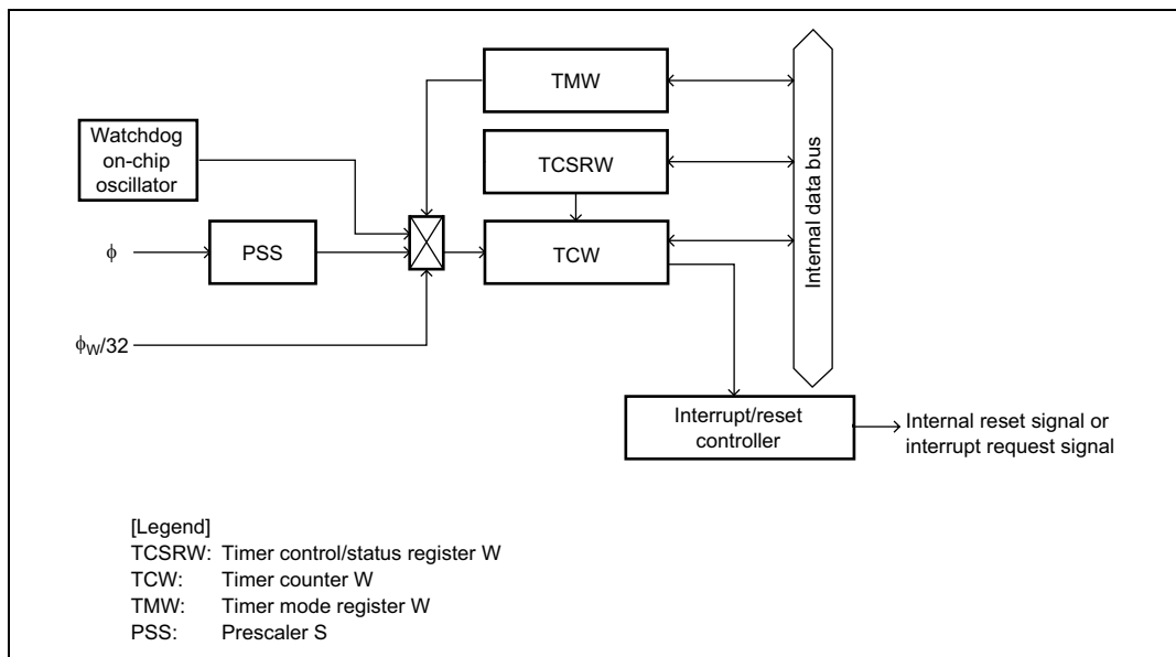
Figure 9.17(2) Block Diagram of Watchdog Timer (H8/38124 Group)
