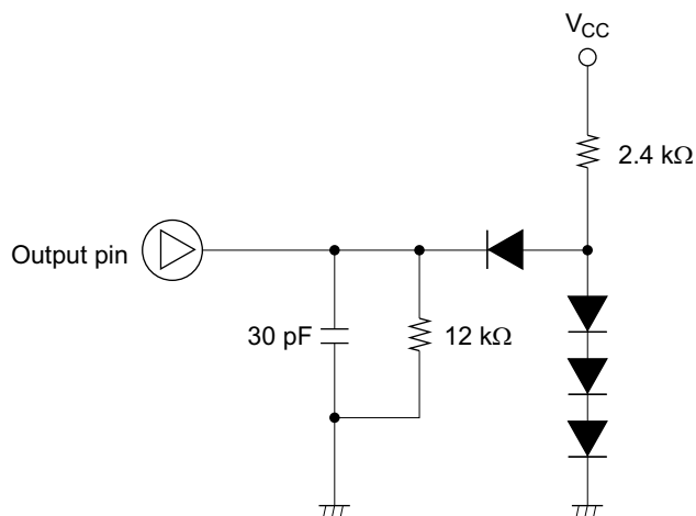
Figure 16.7 Output Load Condition
