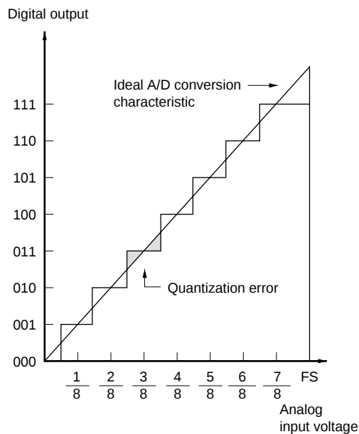
Figure 12.6 A/D Conversion Accuracy Definitions (1)
