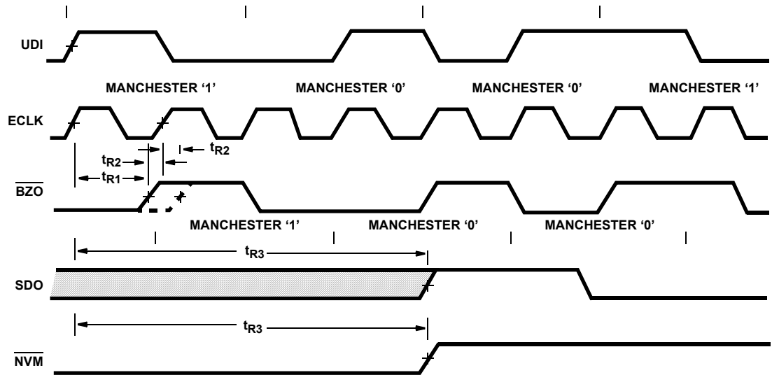
FIGURE 17. REPEATER TIMING
