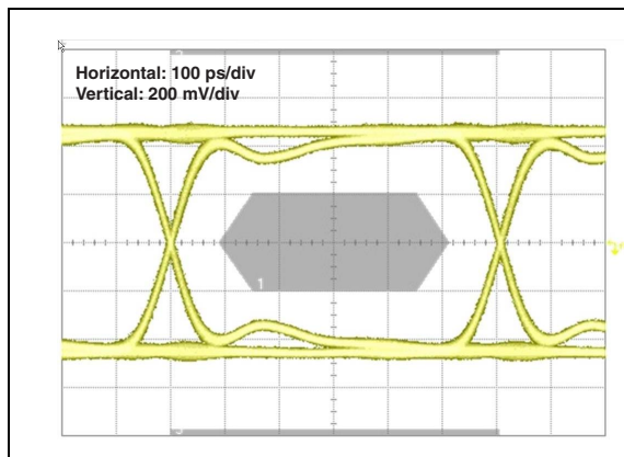
Figure 10. Eye diagram at 1.65 Gbps amplitude 500 mV PCB + HDMIULC6-2P6
