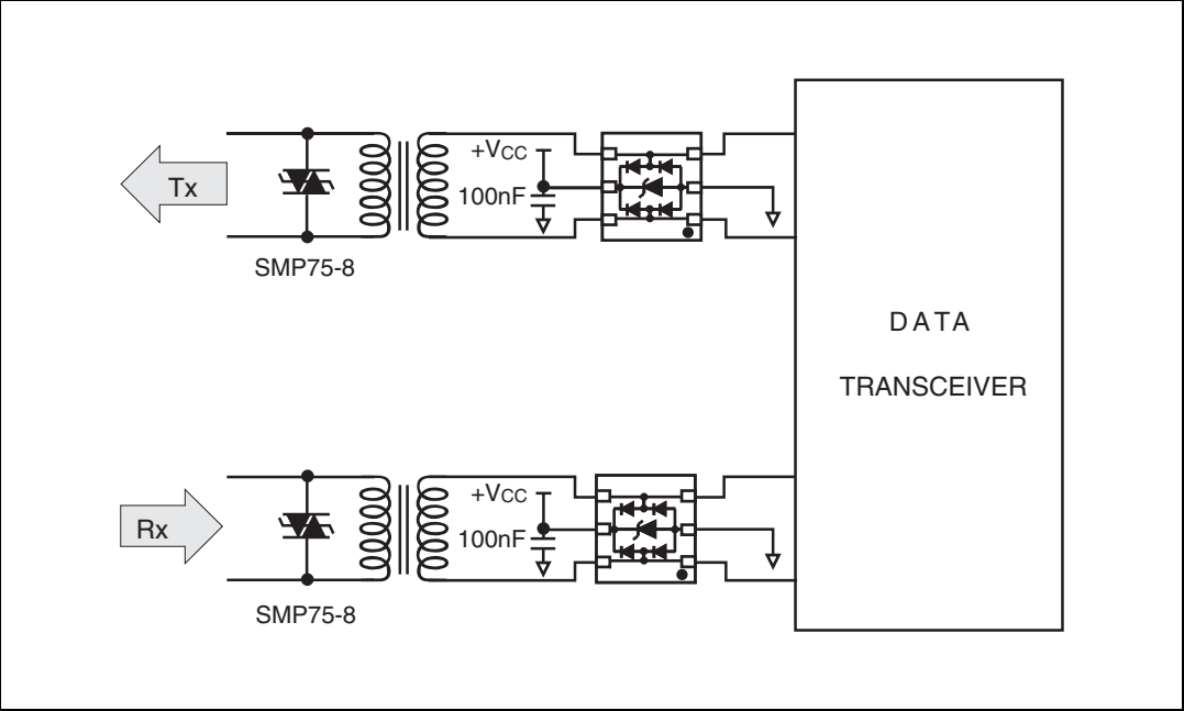
Figure 13. T1/E1/Ethernet protection
