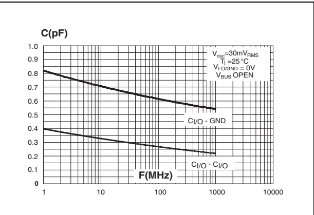
Figure 3. Line capacitance versus frequency (typical values) HDMIULC6-2M6
