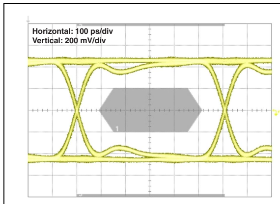
Figure 8. Eye diagram at 1.65 Gbps amplitude 500 mV PCB + HDMIULC6-2M6
