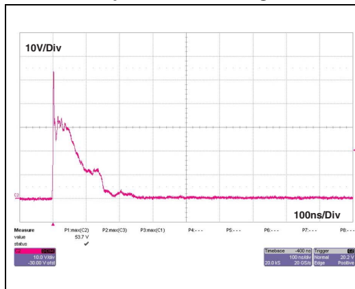
Figure 20. Remaining voltage after the HDMIULC6-2P6 during positive ESD surge
