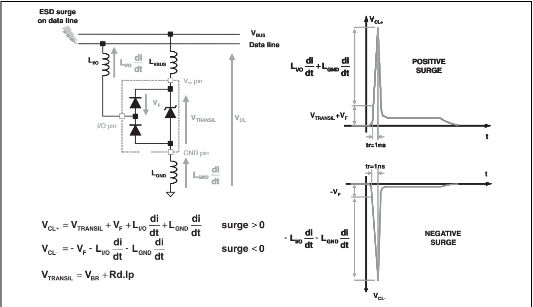
Figure 16. ESD behavior: parasitic phenomena due to unsuitable layout
