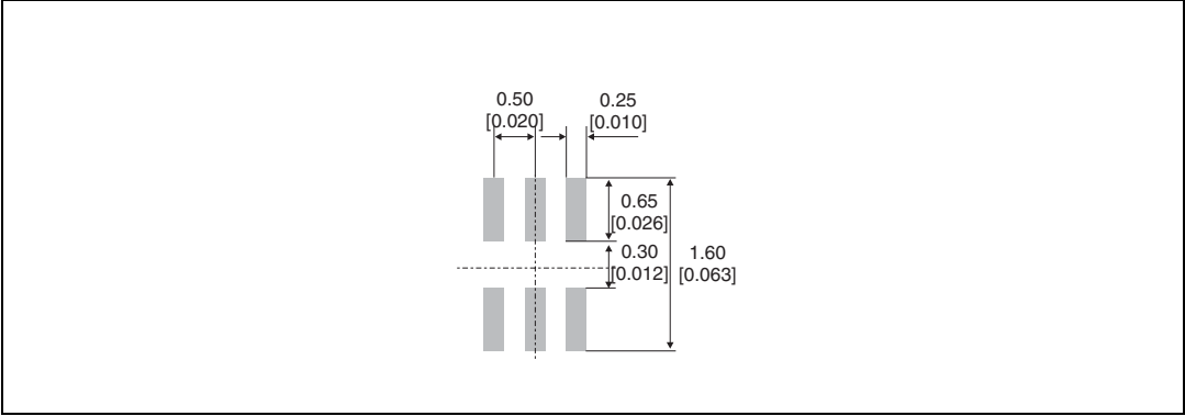
Figure 29. µQFN 6 leads footprint dimensions in mm [inches]
