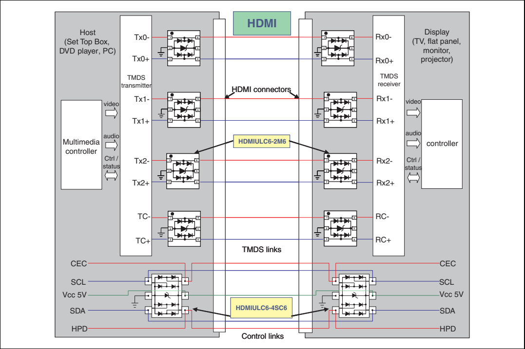
Figure 12. HDMI single link application
