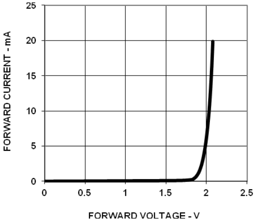
Figure 13 Forward Voltage Vs Current
