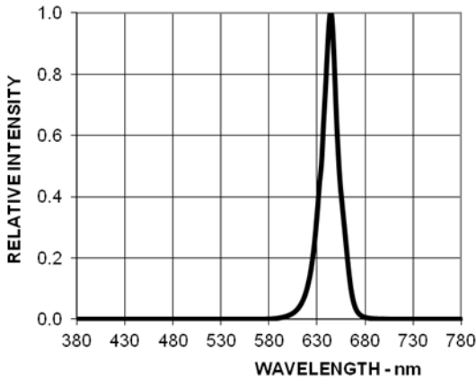
Figure 14 Relative Luminous Intensity Vs Wavelength
