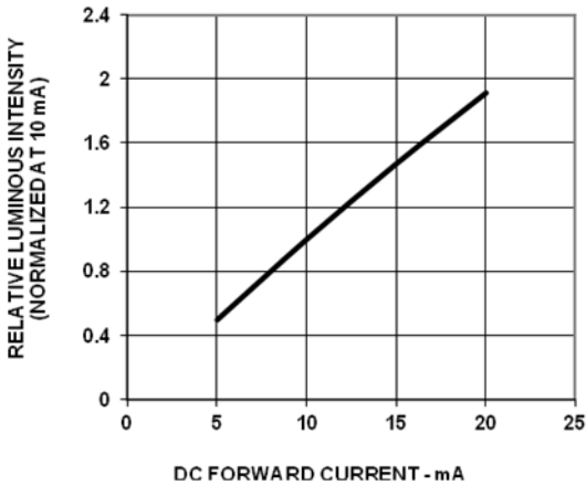
Figure 12 Relative Luminous Intensity Vs Forward Current
