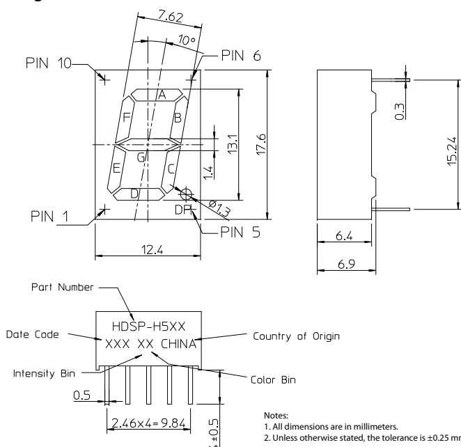
Figure 1 Package Dimension
