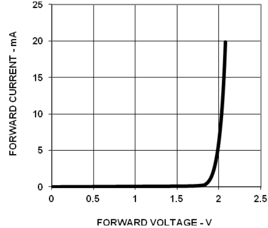
Figure 13 Forward Voltage Vs Current
