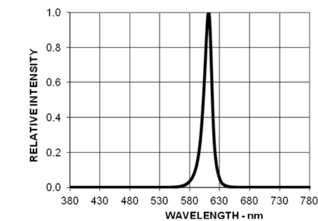
Figure 11 Relative Luminous Intensity Vs Wavelength
