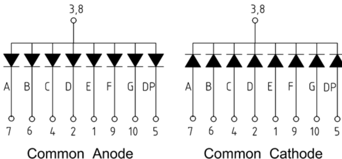
Figure 2 Circuit Diagram
