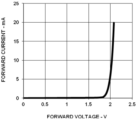
Figure 10 Forward Voltage Vs Current
