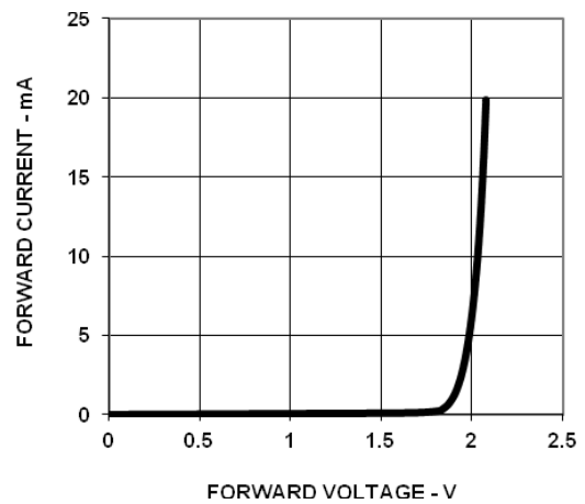
Figure 7 Forward Voltage Vs Current
