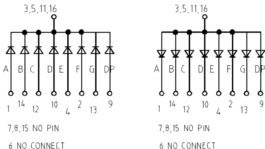
Figure 2 Circuit Diagram
