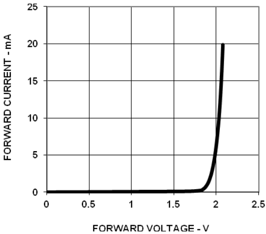
Figure 7 Forward Voltage Vs Current
