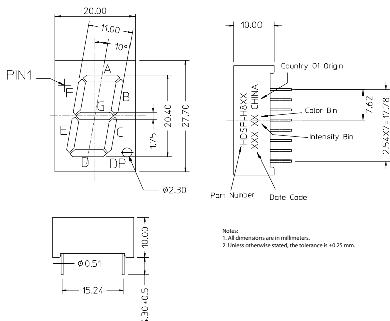
Figure 1 Package Dimension
