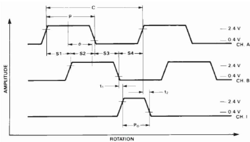
Figure 2. Output waveforms
