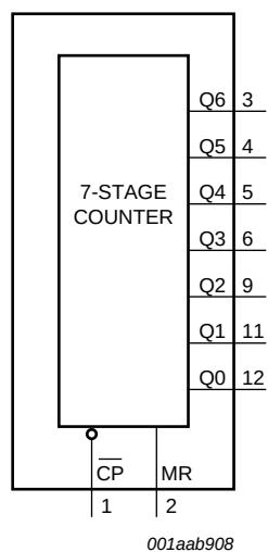
Fig 1. Functional diagram
