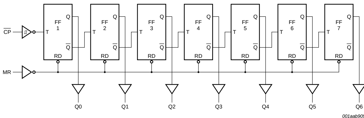
Fig 3. Logic diagram
