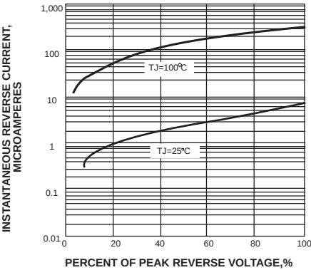
FIG. 4-TYPICAL REVERSE CHARACTERISTICS
