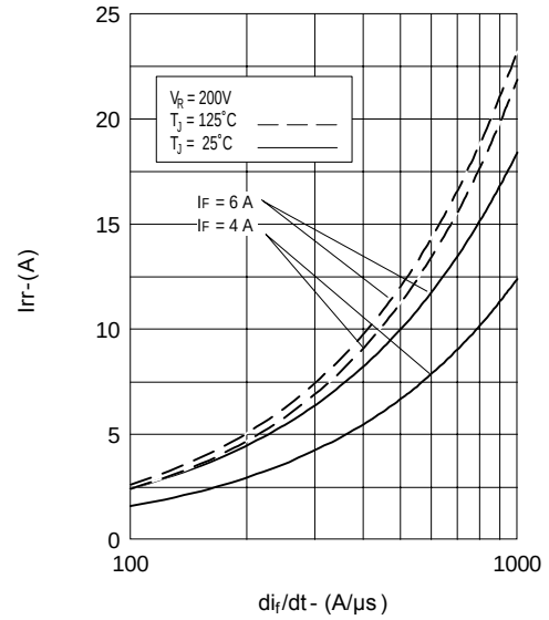
Fig. 6 - Typical Recovery Current Vs. di_I/dt
