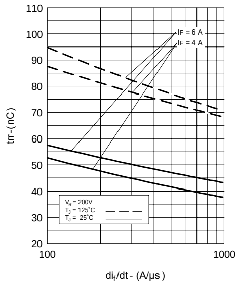
Fig. 5 - Typical Reverse Recovery Vs. di_I/dt
