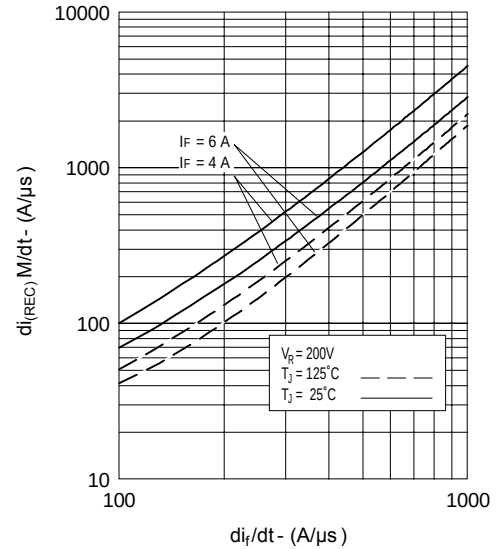
Fig. 7 - Typical di_{(REC)} M/dt vs. di_I/dt
