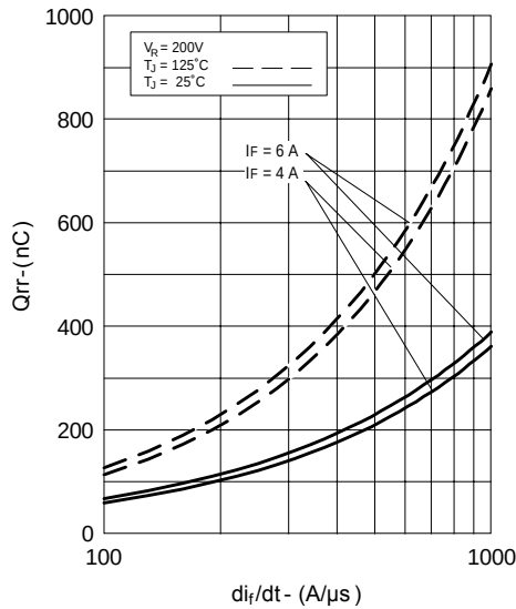
Fig. 8 - Typical Stored Charge vs. di_I/dt
