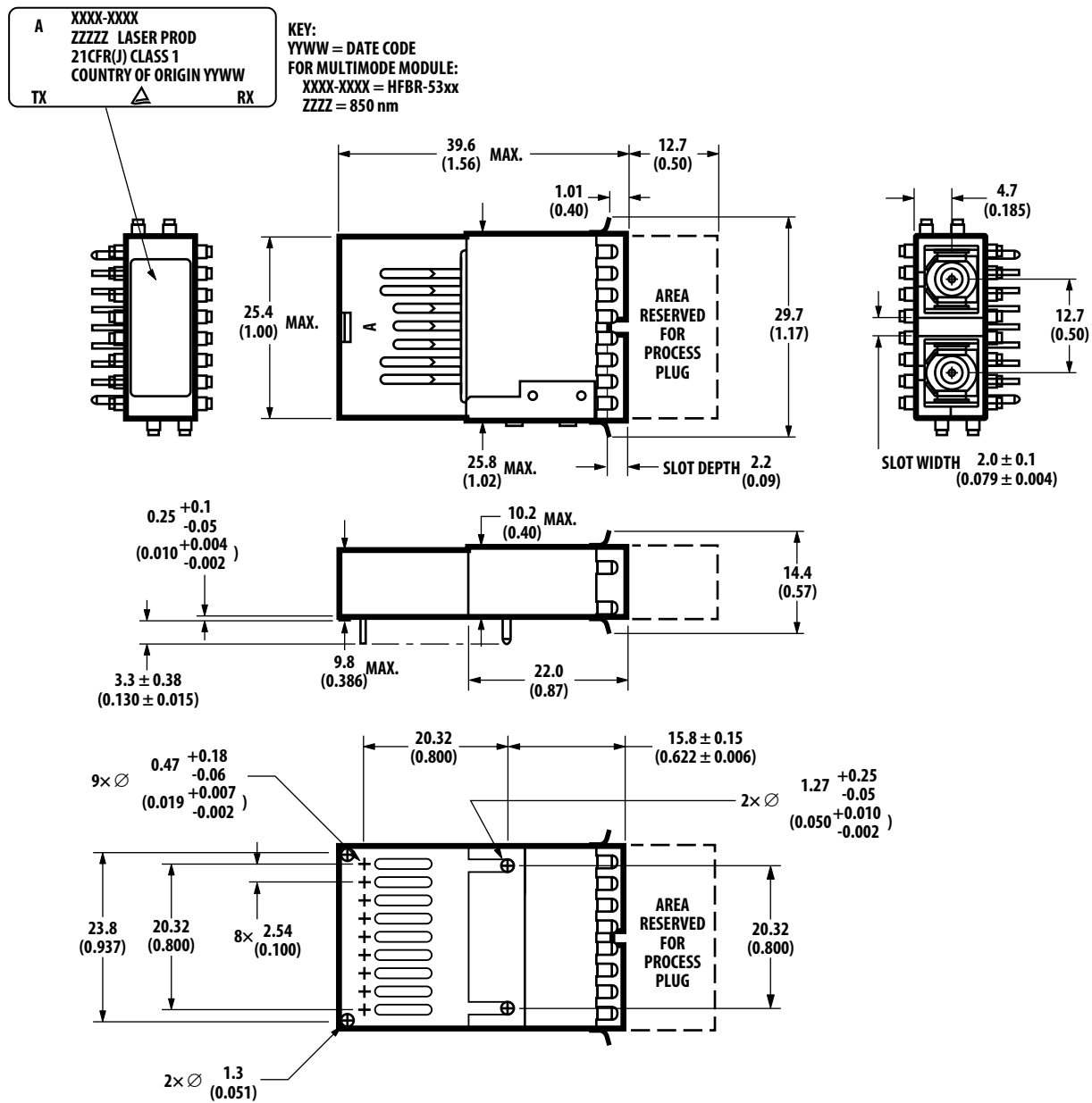
Figure 7. Package outline for HFBR-53A5VFMZ
