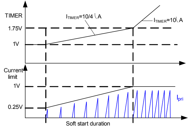
Figure 6: Soft-Start
