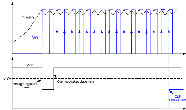
Figure 8: Overload Protection
