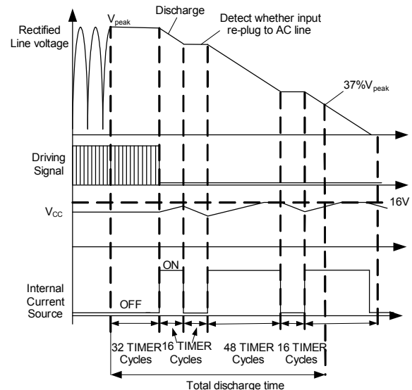
Figure 9: X-Cap Discharger
