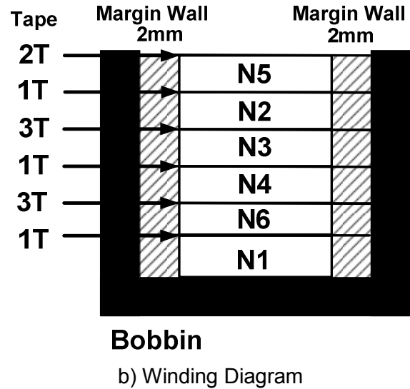
Figure 17: Transformer Structure
