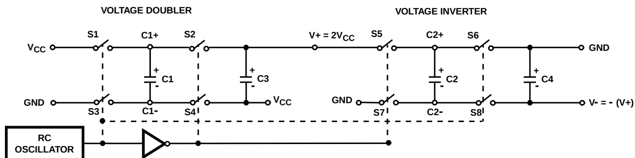
FIGURE 1. CHARGE PUMP
