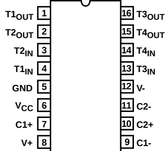
HIN204 (SOIC) TOP VIEW
