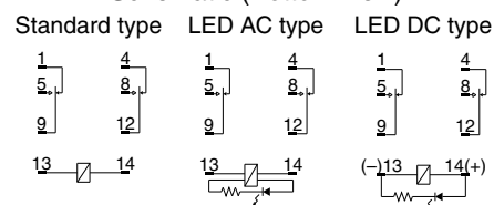
Schematic (Bottom view)
