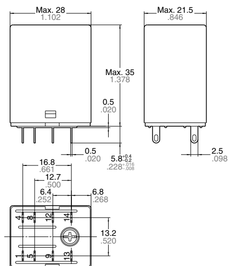
External dimensions
