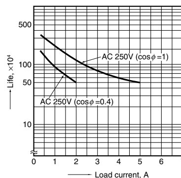
2-(1). Life curve (2 Form C)
