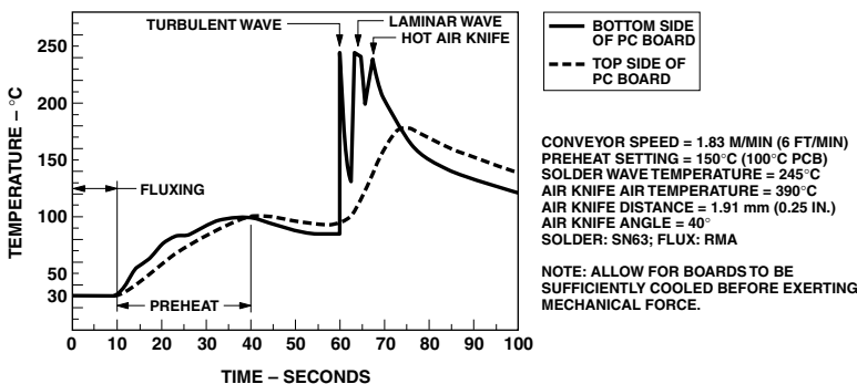
Figure 17. Recommended wave soldering profile.
