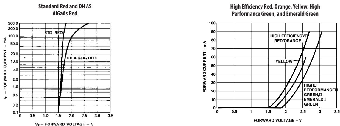
Figure 2. Forward current vs. forward voltage (non-resistor lamp).
