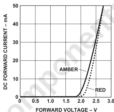
Figure 3b. Forward current vs. forward voltage for option -xxTxx red, and option -xxRxx and -xxSxx amber.
