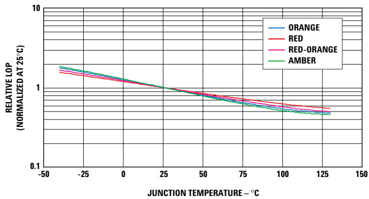
Figure 9. Relative light output vs. junction temperature
