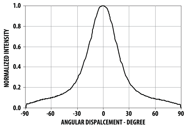
Figure 6. Radiation pattern-Minor Axis
