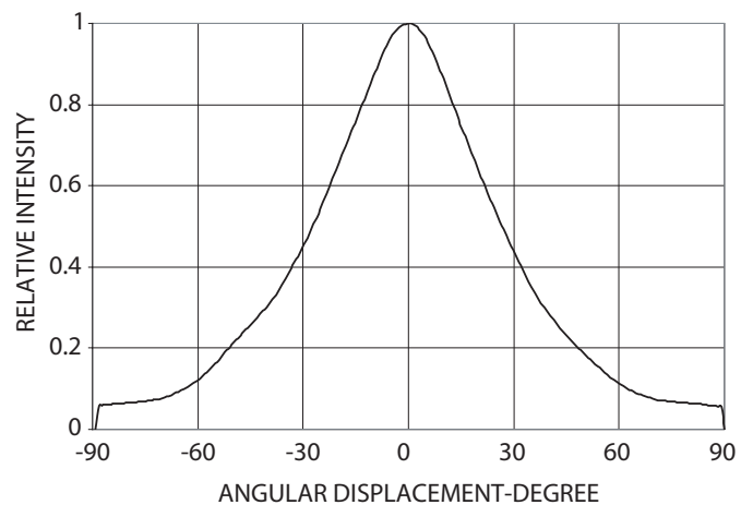
Figure 11: Radiation pattern-Minor Axis
