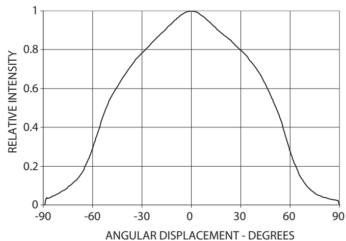
Figure 10: Radiation pattern-Major Axis
