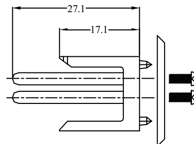
Keying Pin
