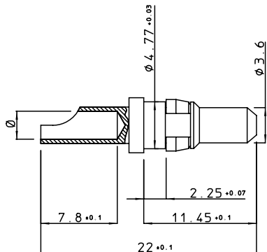
pin contact
