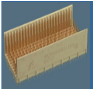
Millipacs™ HM2P88PNA124GF
