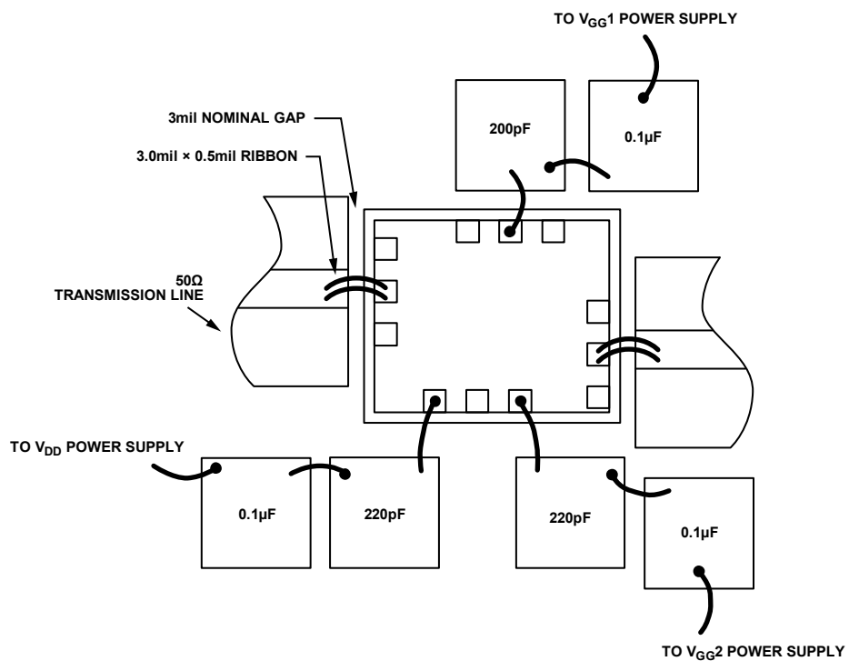
Figure 24. Assembly Diagram
