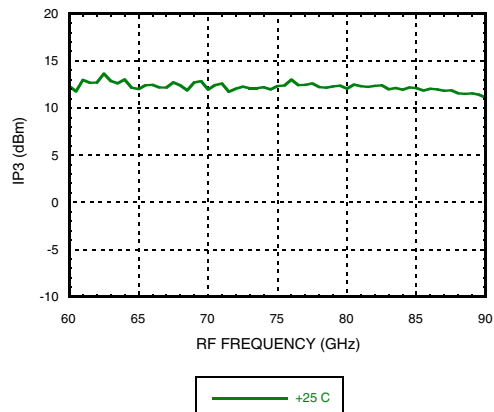
Upconverter Performance Input IP3, USB
