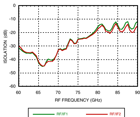
RF/IF Isolation
